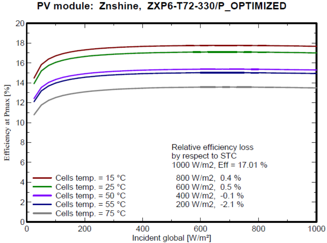
Figure 2 PVsyst Efficiency Curves for the Optimized ZXP6-T72-330/P and ZXP6-T72-325/P PAN File
