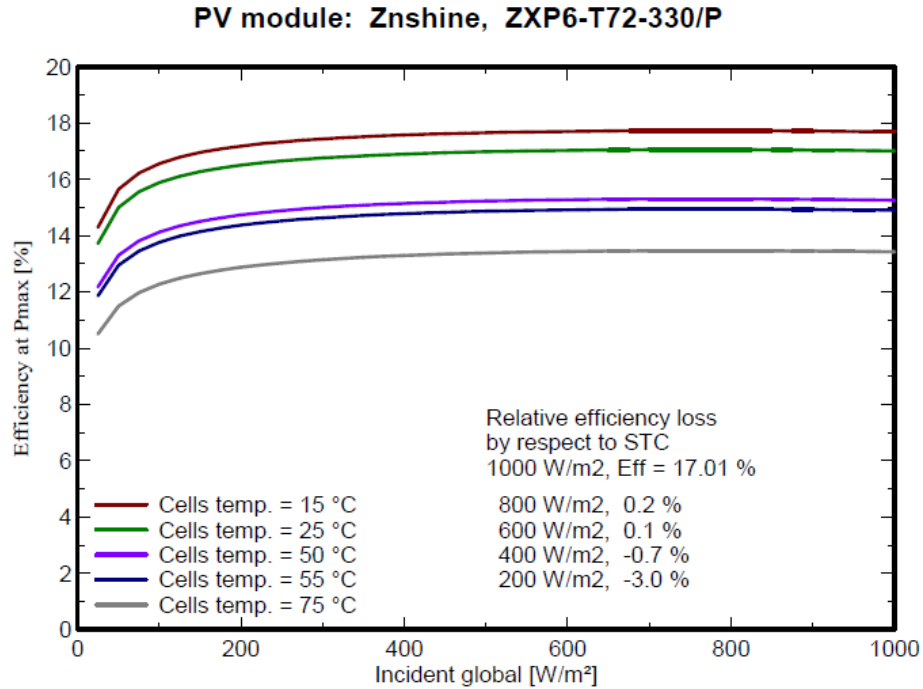
Figure 1 PVsyst Efficiency Curves for the Base Case ZXP6-T72-330/P and ZXP6-T72-325/P
